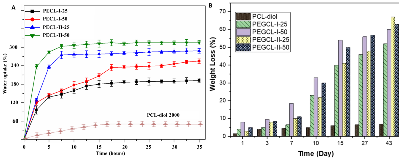
Figure 5. Properties of plain copolymer nanofibers relative to PCL-diol (2000) prepolymer nanofibers at 37°C: (A) Water uptake capacity; (B) Weight loss (%).
