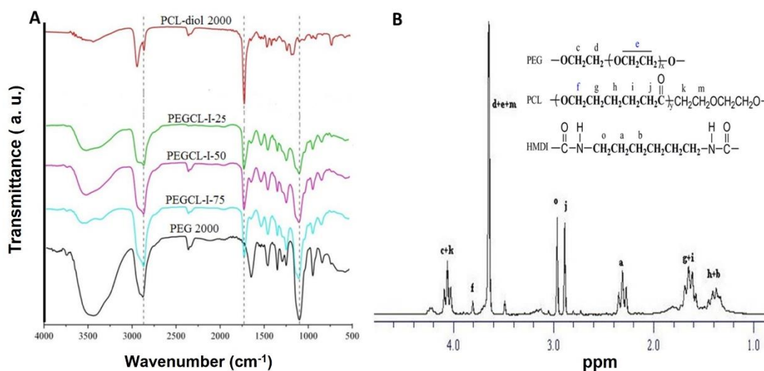
Figure 2. Copolymer characterization: (A) FT-IR spectra of selected samples and (B) ^1\text{H-NMR} spectrum of a representative copolymer, PEGCL-I-50.
