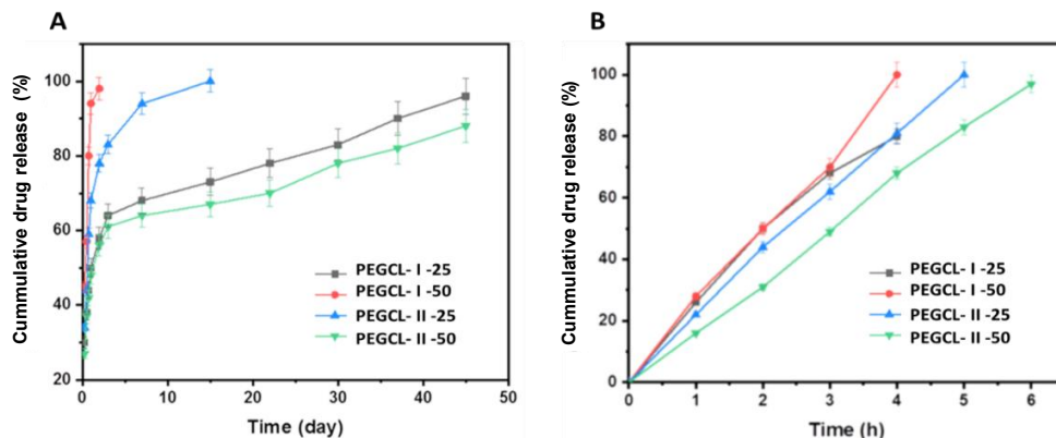
Figure 9. Chlorhexidine release profiles at: (A) pH 7.4 and (B) pH 4 at 37°C.
